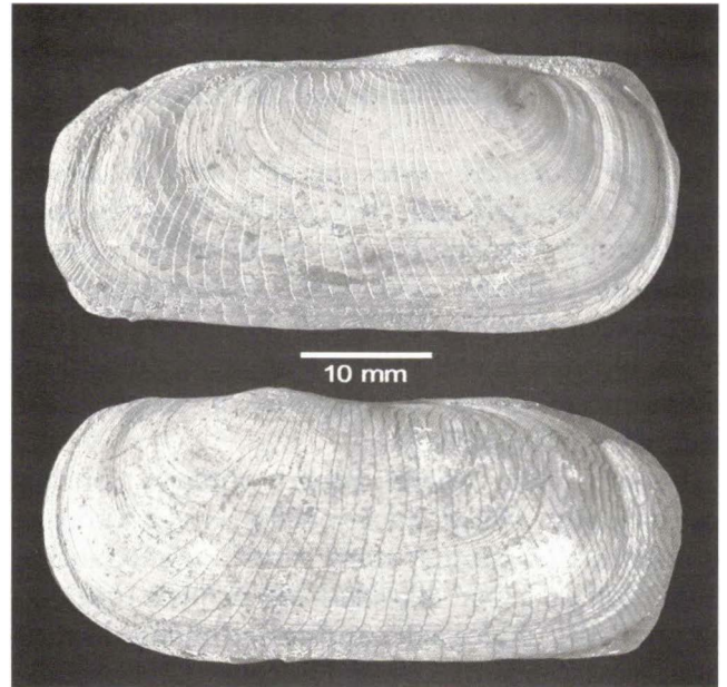
Figure 9 Lectotype of Solen candidus Brocchi 1814, Valle Andona, upper Pliocene (Piacenzian), Brocchi collection, MSNMi13351.
